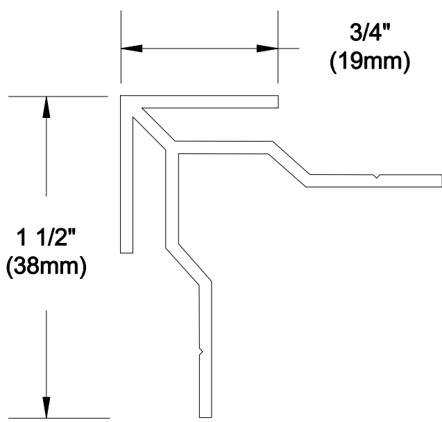
CR-AX5 OUTSIDE CORNER
