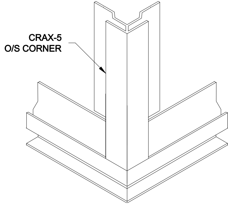
12B BASE OUTSIDE CORNER, OPTION 2
