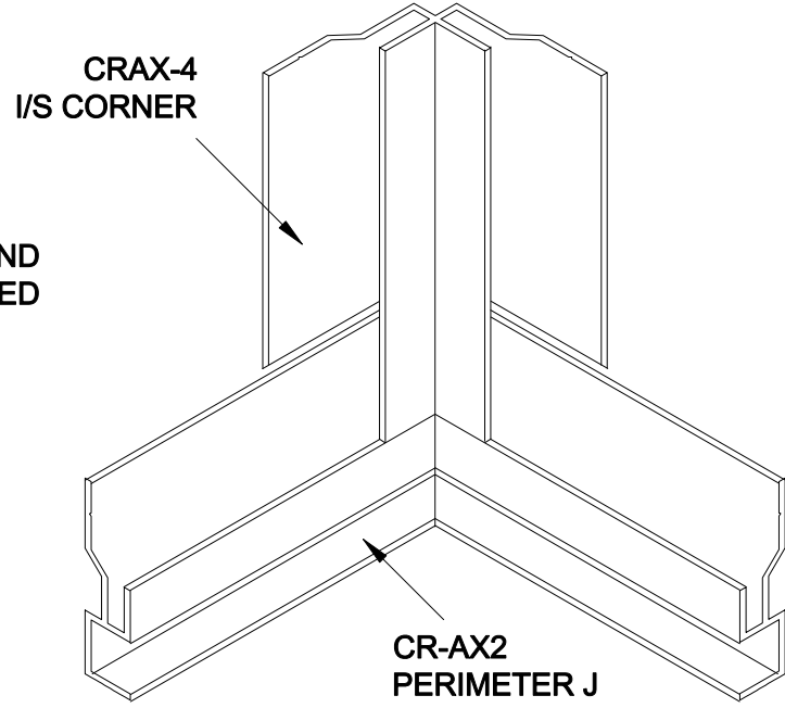
11B BASE INSIDE CORNER, OPTION 2
