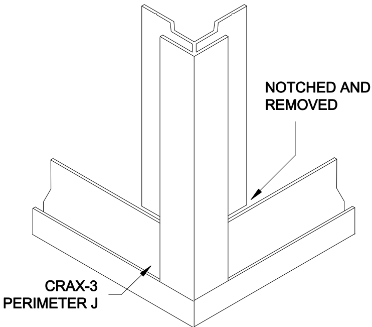
12A BASE OUTSIDE CORNER, OPTION 1
