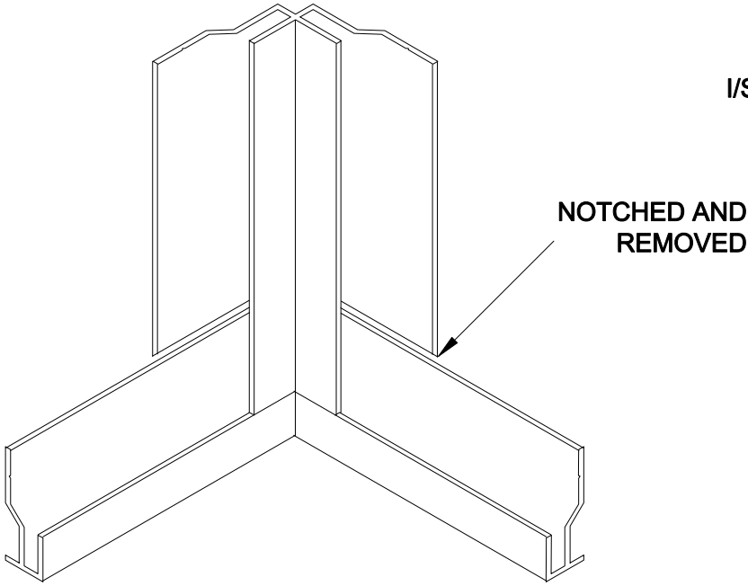
11A BASE INSIDE CORNER, OPTION 1
