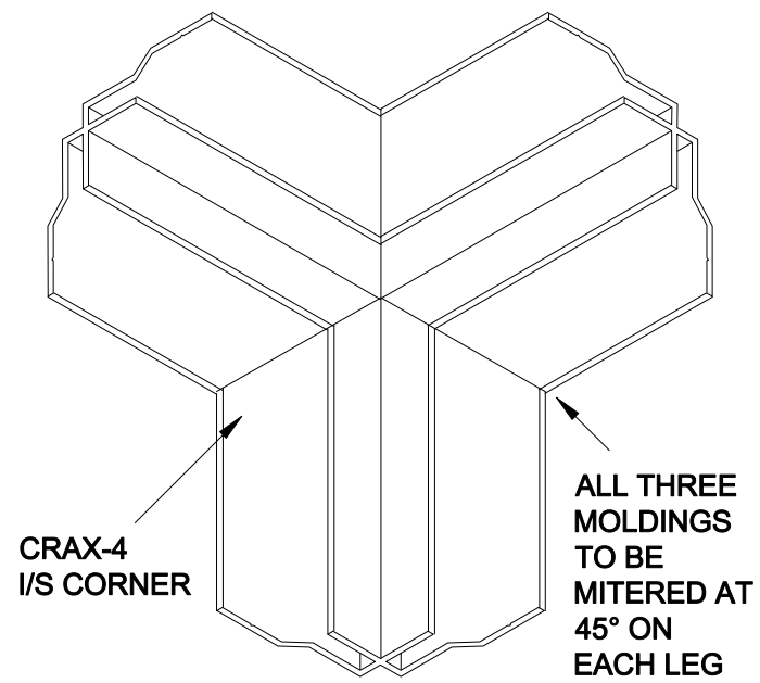
17 THREE WAY INSIDE CORNER
