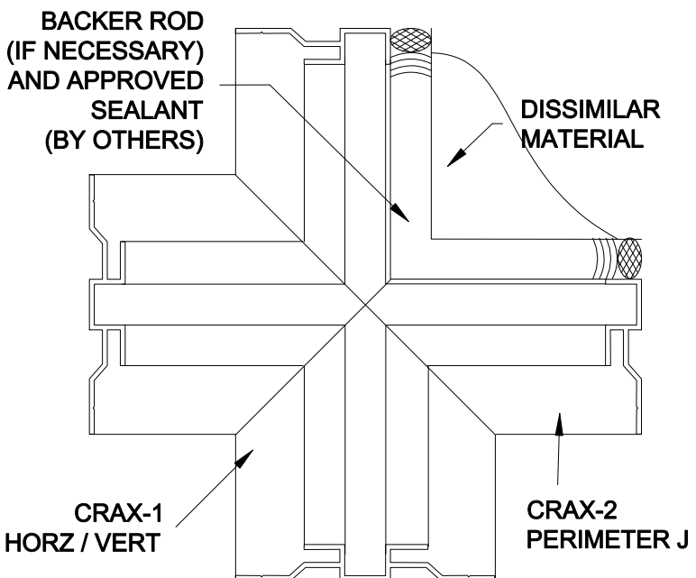
16B DISSIMILAR MATERIAL CORNER, OPT. 2
