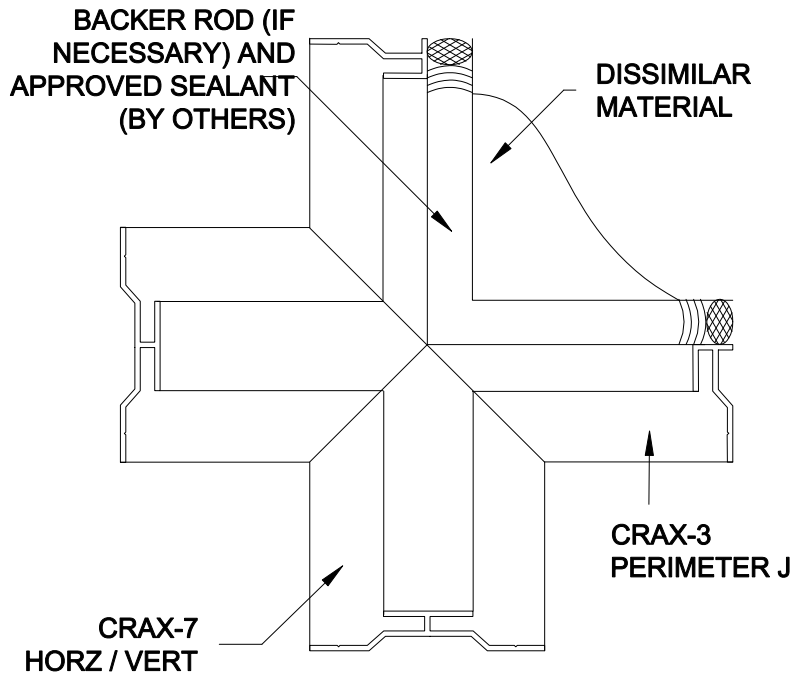
16A DISSIMILAR MATERIAL CORNER, OPT. 1
