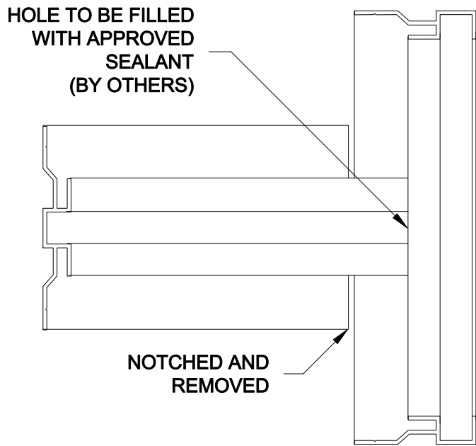
15B HORZ TERMINATION ONLY, OPTION 2
