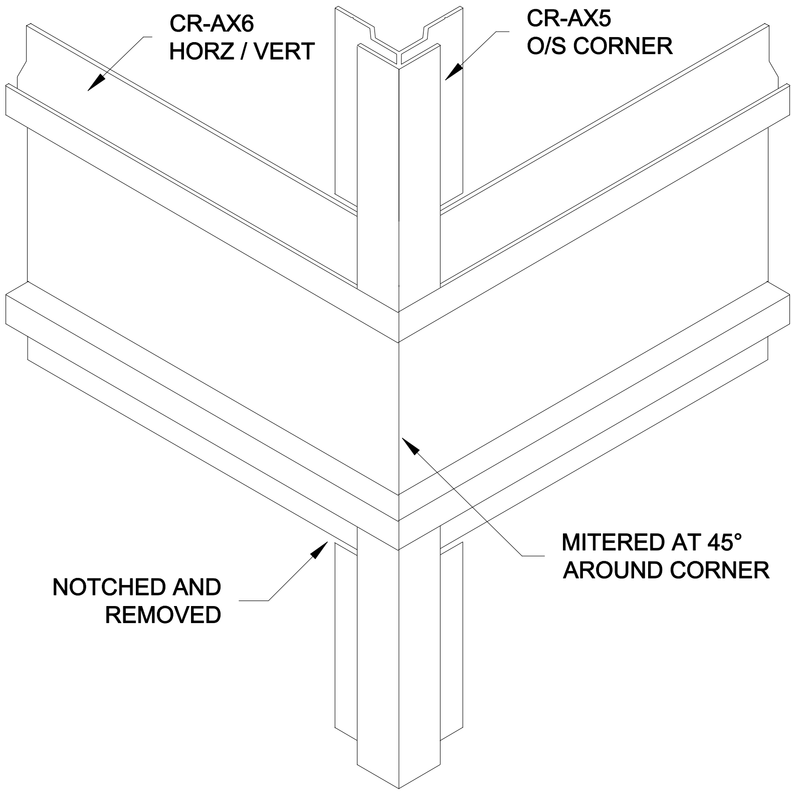
19D OUTSIDE CORNER, OPTION 4
