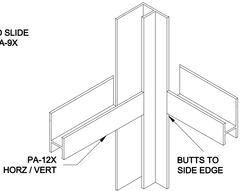
18B INSIDE CORNER, OPTION 2
