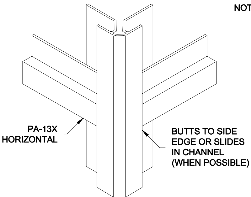
19A OUTSIDE CORNER, OPTION 1
