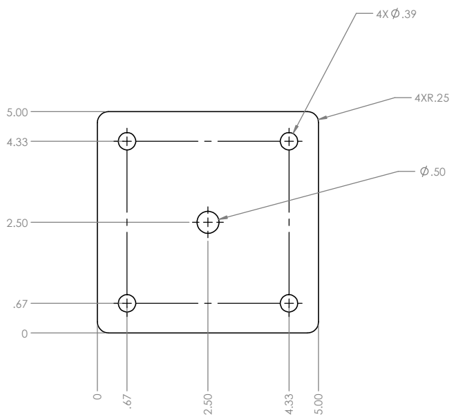
BASEPLATE DETAIL
