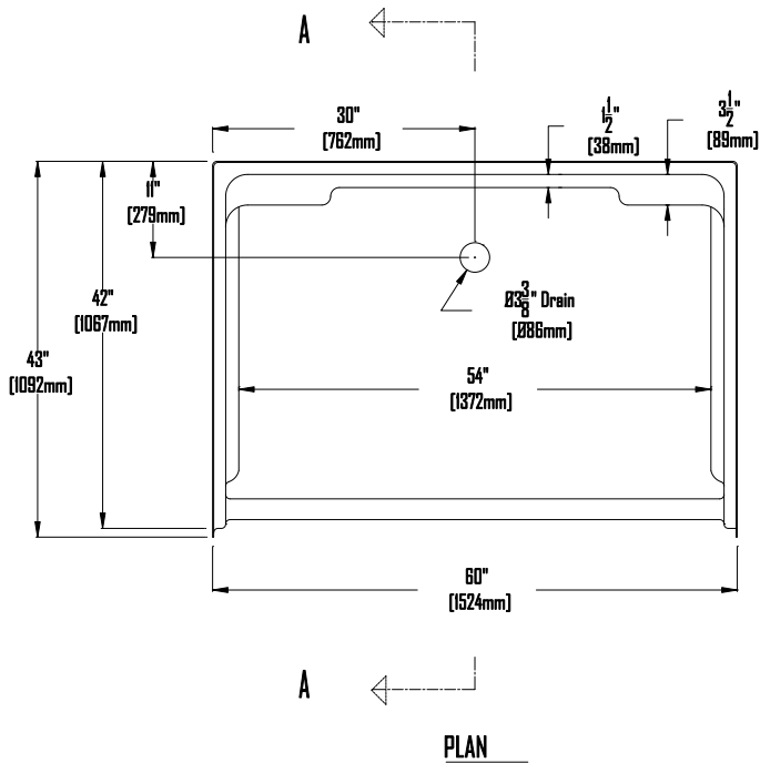
60" [1524mm] Convertible Shower Stall
