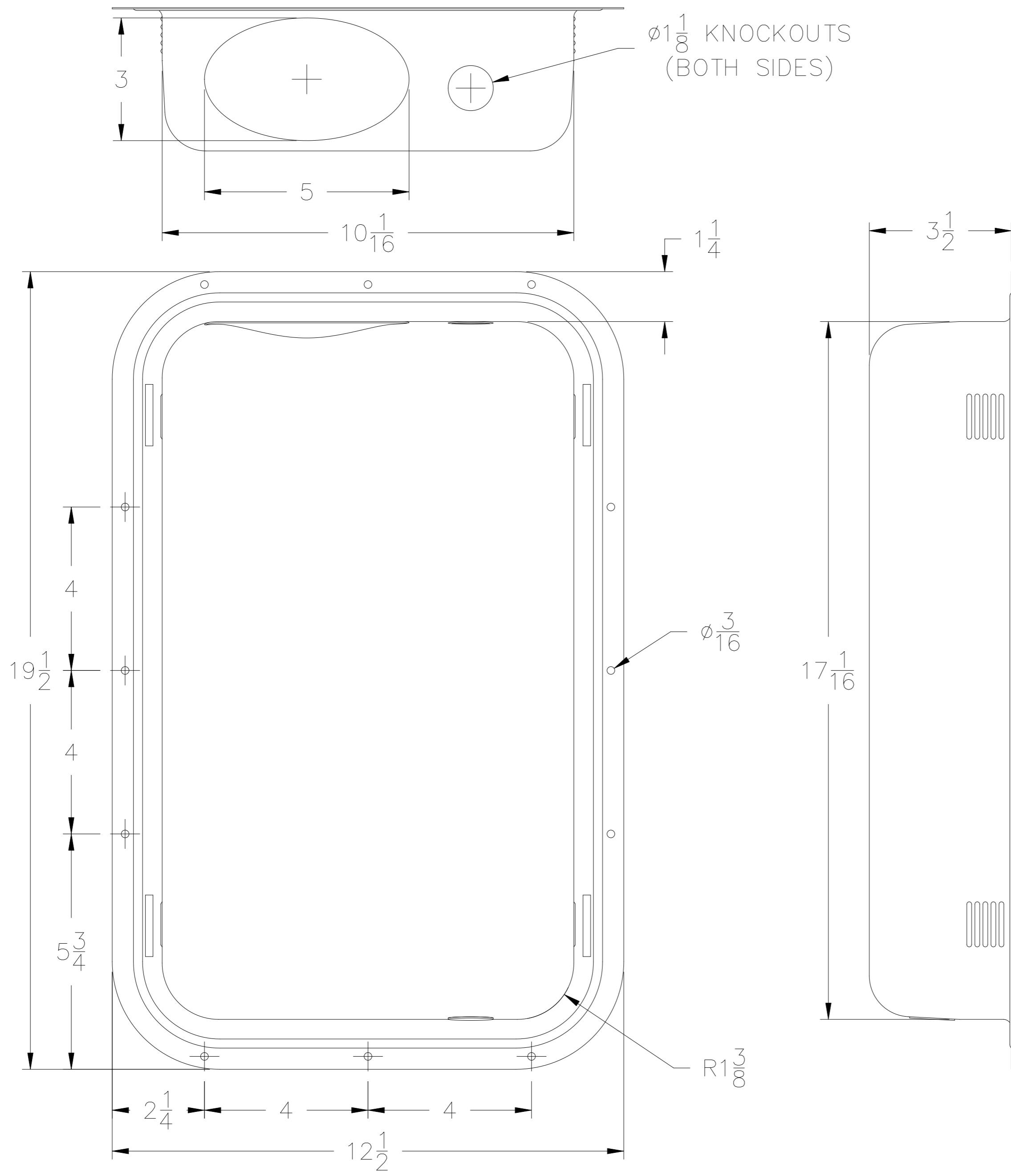
DBX1000M BOX DIMENSION VIEW
