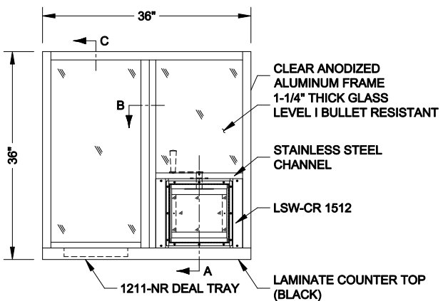
FRONT VIEW SPECIAL XW-LS 3636
