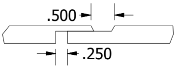
LAP DETAIL
