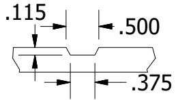
GROOVE DETAIL
