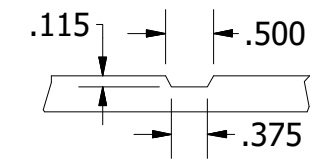
GROOVE DETAIL
