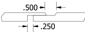
LAP DETAIL
