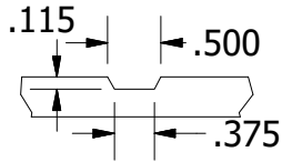
GROOVE DETAIL
