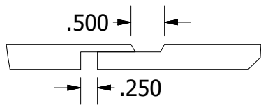
LAP DETAIL
