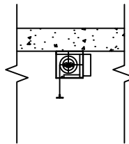
B1 - EXPOSED WITH TOP SIDE TO SLAB MOUNT
