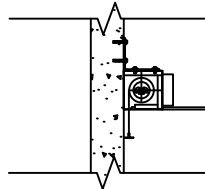
A2 - FLUSH CEILING WITH FACE MOUNT
