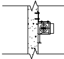
A1 - HEADBOX EXPOSED WITH FACE MOUNT
