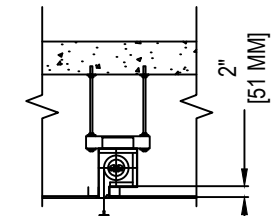
C4 - DOWNSTAND WITH UNISTRUT MOUNT
