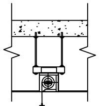
C2 - FLUSH CEILING WITH UNISTRUT MOUNT
