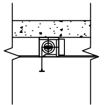
B2 - FLUSH CEILING WITH TOP SIDE TO SLAB MOUNT
