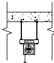
C1 - HEADBOX EXPOSED WITH UNISTRUT MOUNT
