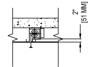
B4 - DOWNSTAND WITH TOP SIDE TO SLAB MOUNT
