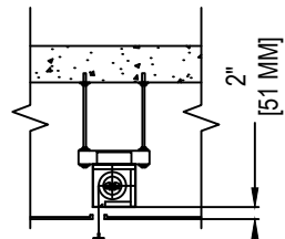
C3 - SHADOW GAP CEILING WITH UNISTRUT MOUNT
