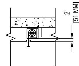
B3 - SHADOW GAP CEILING WITH TOP SIDE TO SLAB MOUNT
