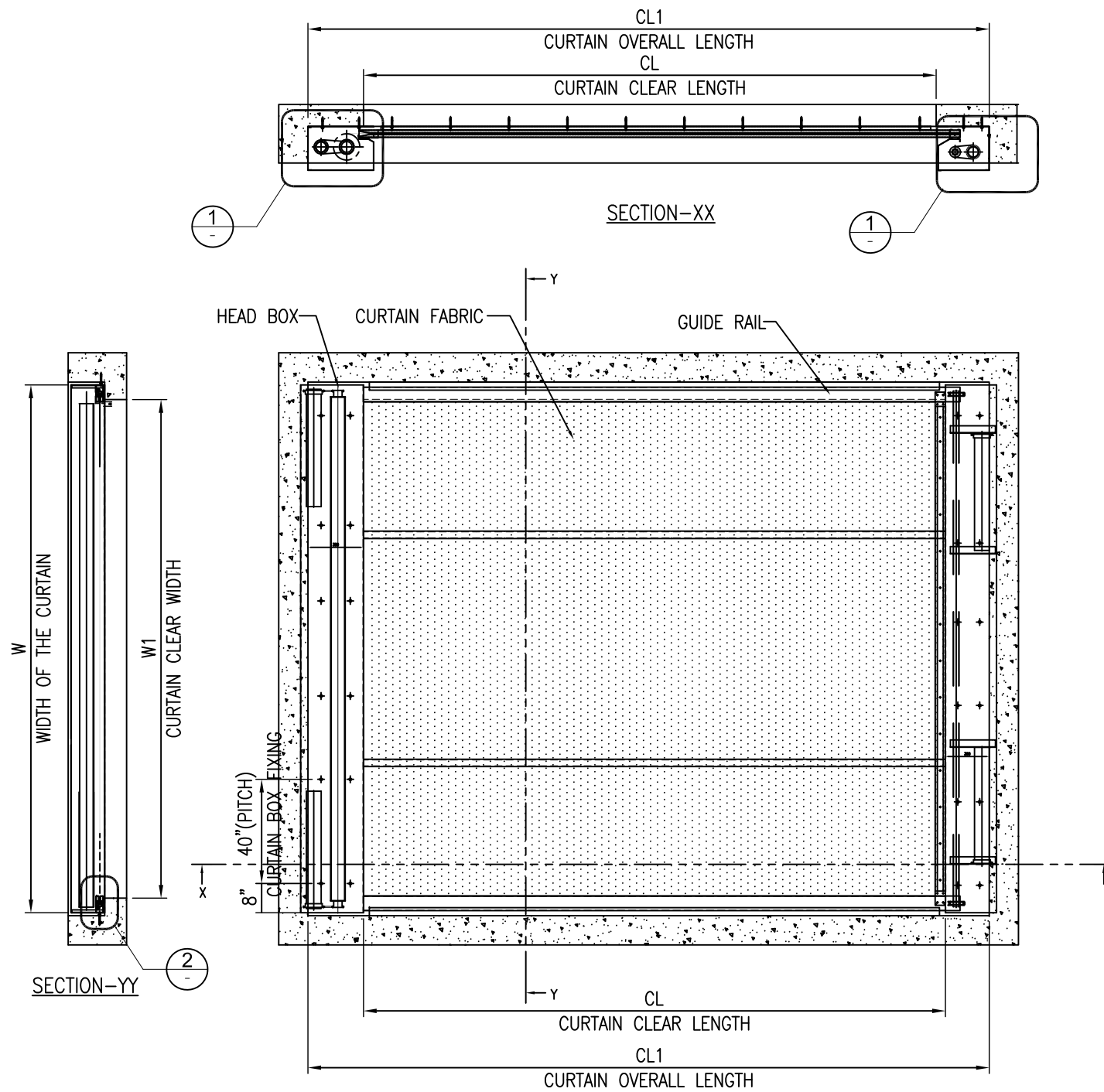
CURTAIN PLAN
