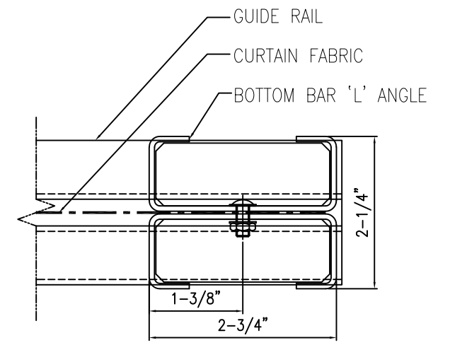
ENLARGED DETAIL - BOTTOM BAR
