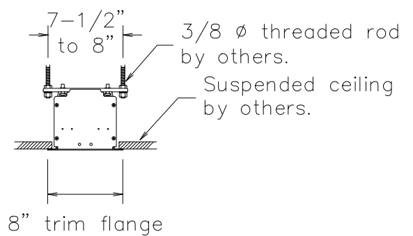
Mounting Details
