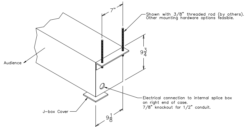
DRAPER SIGNATURE/E/V (small) Isometric Mounting Detail
