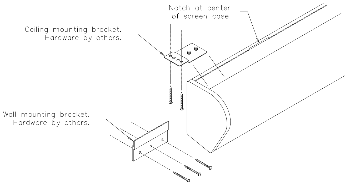
Mounting Detail
