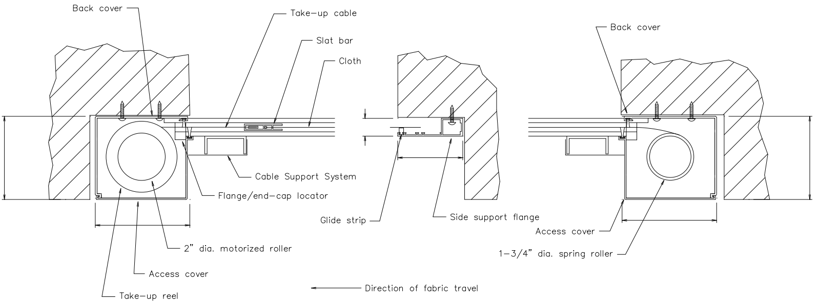
DRAPER SKYLIGHT FLEXSHADE Typical Outside Installation – Boxes Down
