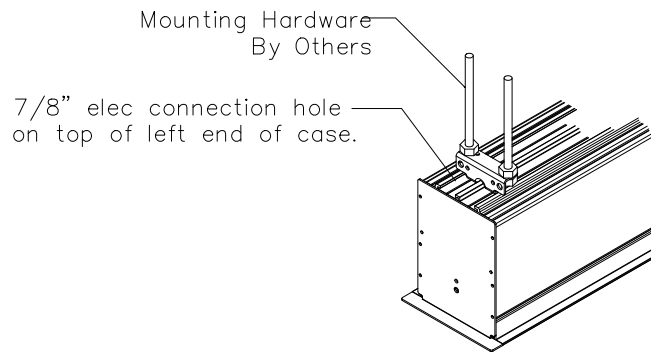
Mounting Detail
