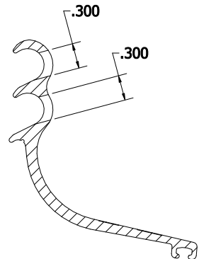
SECTION VIEW AF-AF SCALE 1.25
