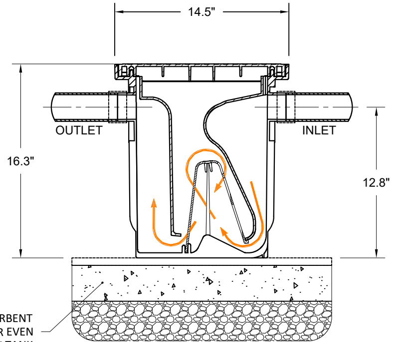
ON-FLOOR INSTALLATION
