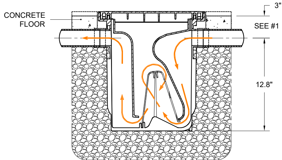
IN-FLOOR INSTALLATION
