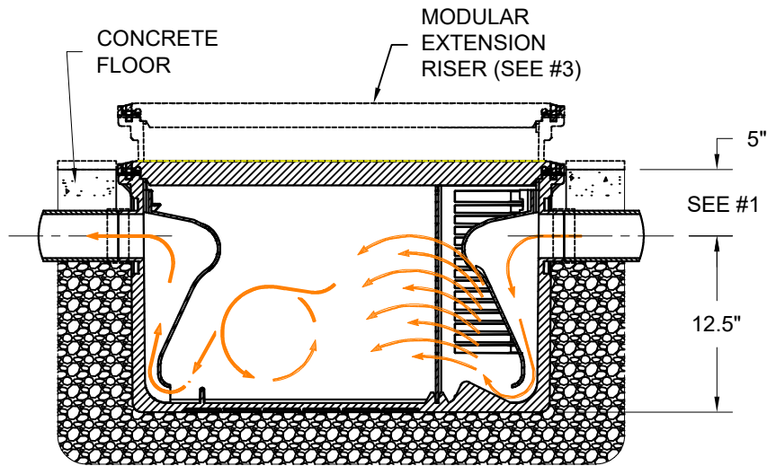
IN-FLOOR INSTALLATION
