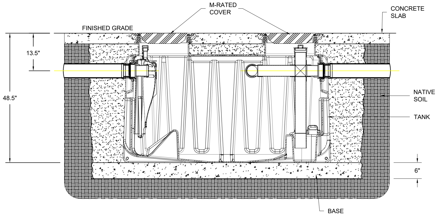
IN-GROUND INSTALLATION-NON TRAFFIC RATED
