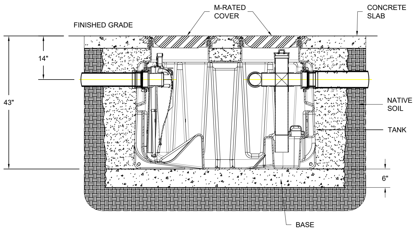
IN-GROUND INSTALLATION-NON TRAFFIC RATED
