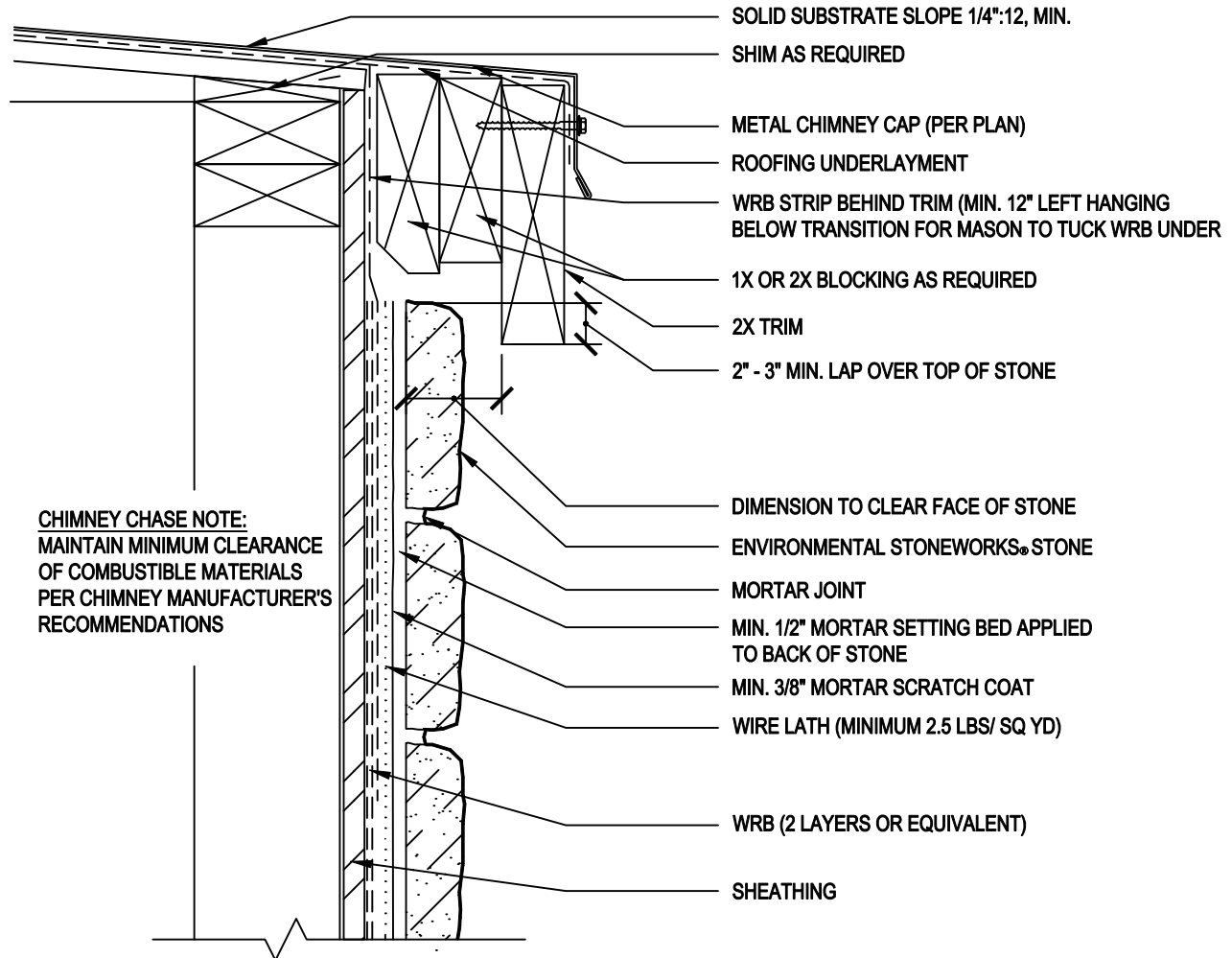
SIDE VIEW
