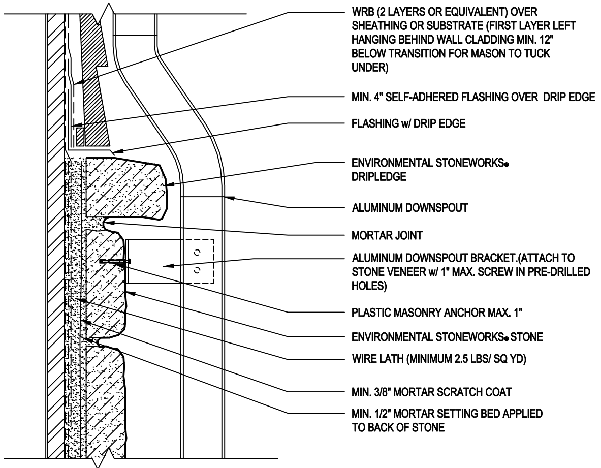
SIDE VIEW
