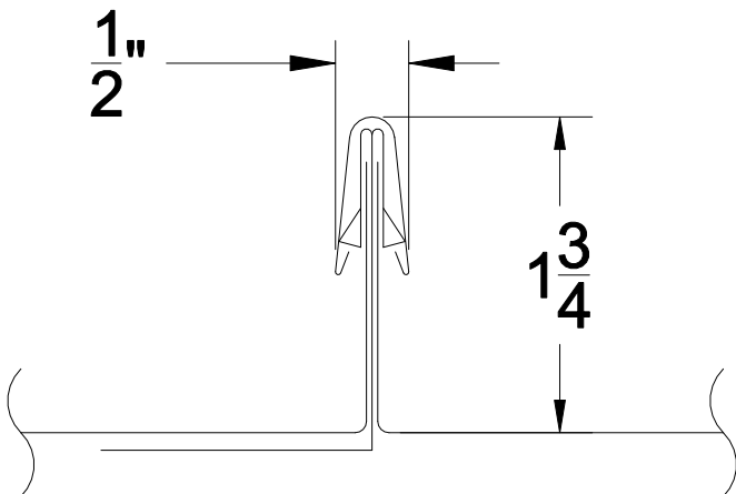
1 3/4" SEAM WITH CAP AND CLIP
