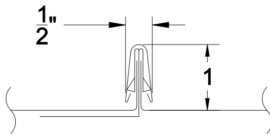
1" SEAM WITH CAP AND CLIP 1 3/4" SEAM WITH CAP AND CLIP
