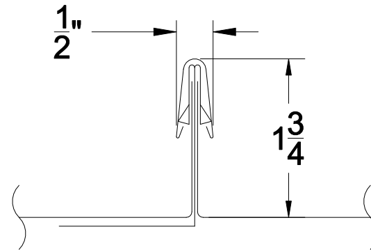
1" SEAM WITH CAP AND CLIP 1 3/4" SEAM WITH CAP AND CLIP
