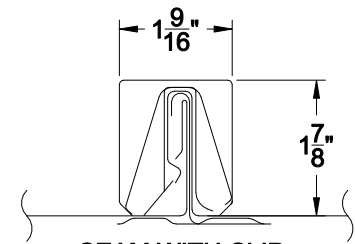
SEAM WITH CLIP, BUTTERFLY CLIP,
