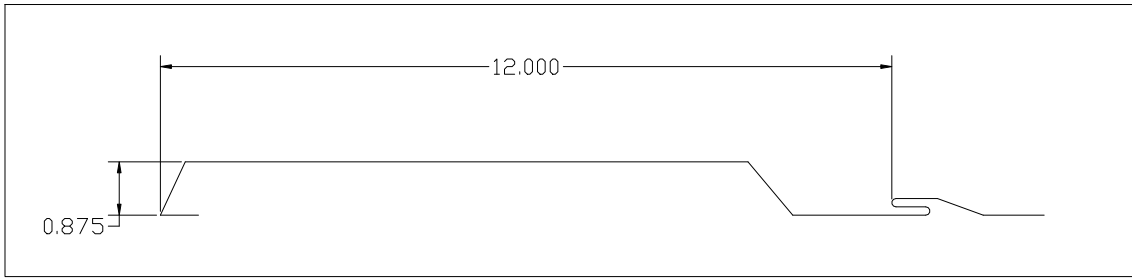
Side Lap Detail
