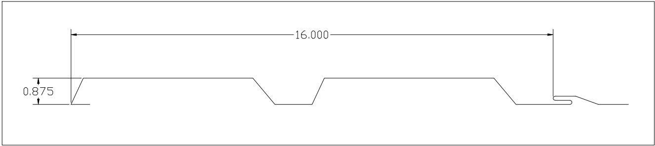
Side Lap Detail
