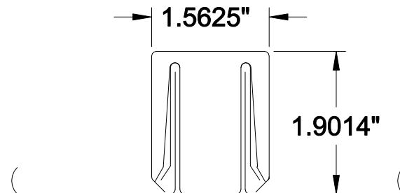
SEAM WITH CAP AND CLIP
