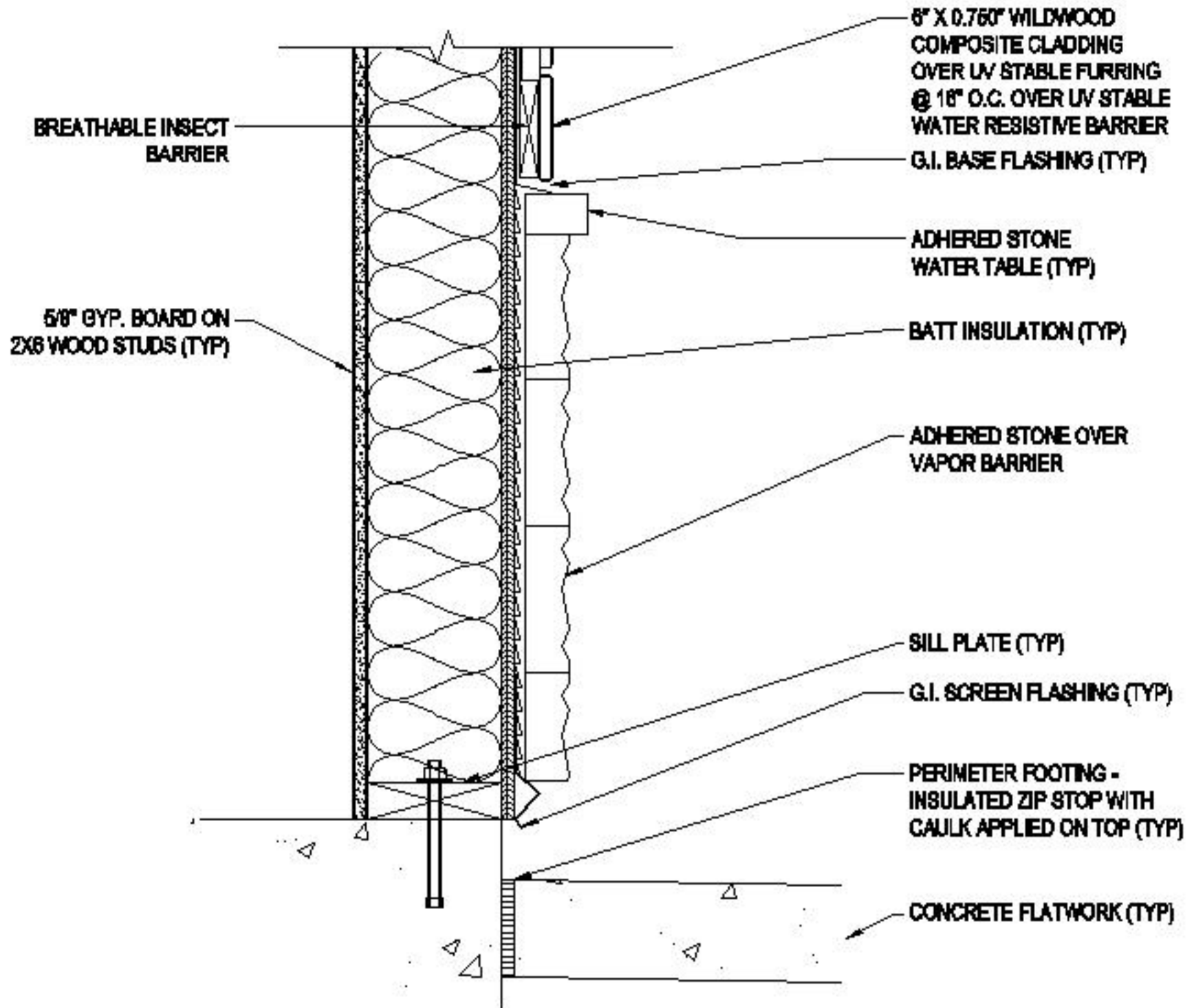
BASE WALL DETAIL
