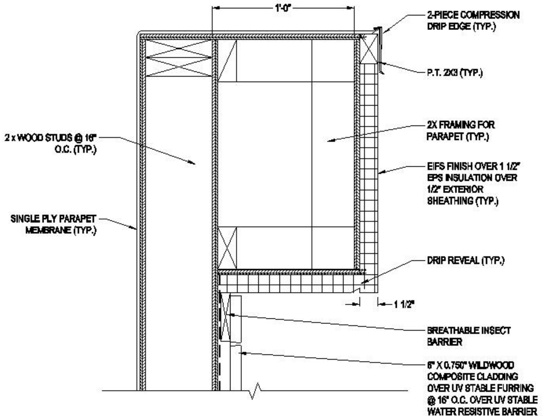
PARAPET DETAIL
