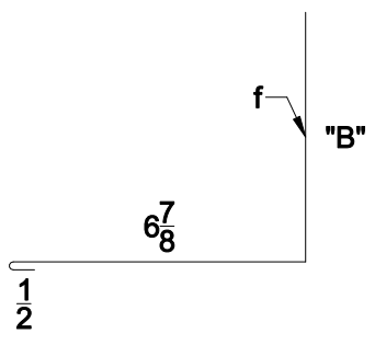
"SR1" BASE ROOF FLASH
