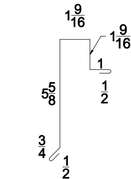
"FSS15-02" GABLE TRIM
