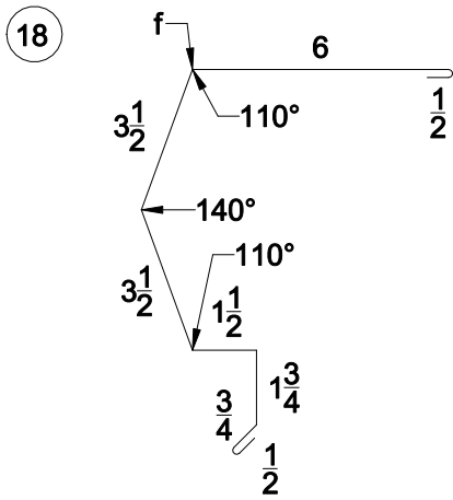
"GT2" GABLE TRIM
