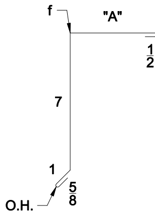
"SS3-03-3" GABLE TRIM
