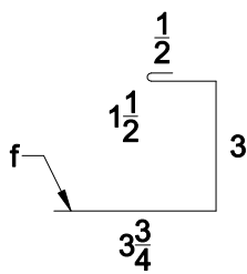
"SS3-03-2" GABLE FILLER
