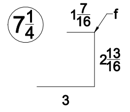
"SS3-01-2" CEE CLOSURE
