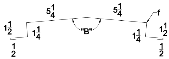
"SS3-01-1" RIDGE CAP
