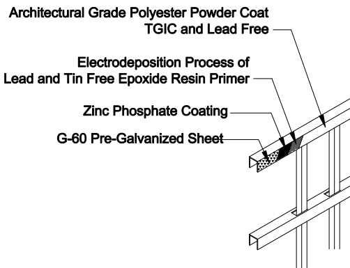
EX-107 Bracket
