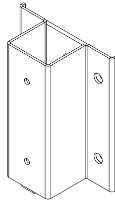
(Isometric View)
