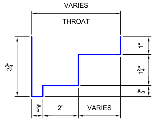
HEAD DETAIL "H1"
