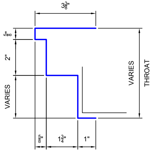
JAMB DETAIL "J1"
