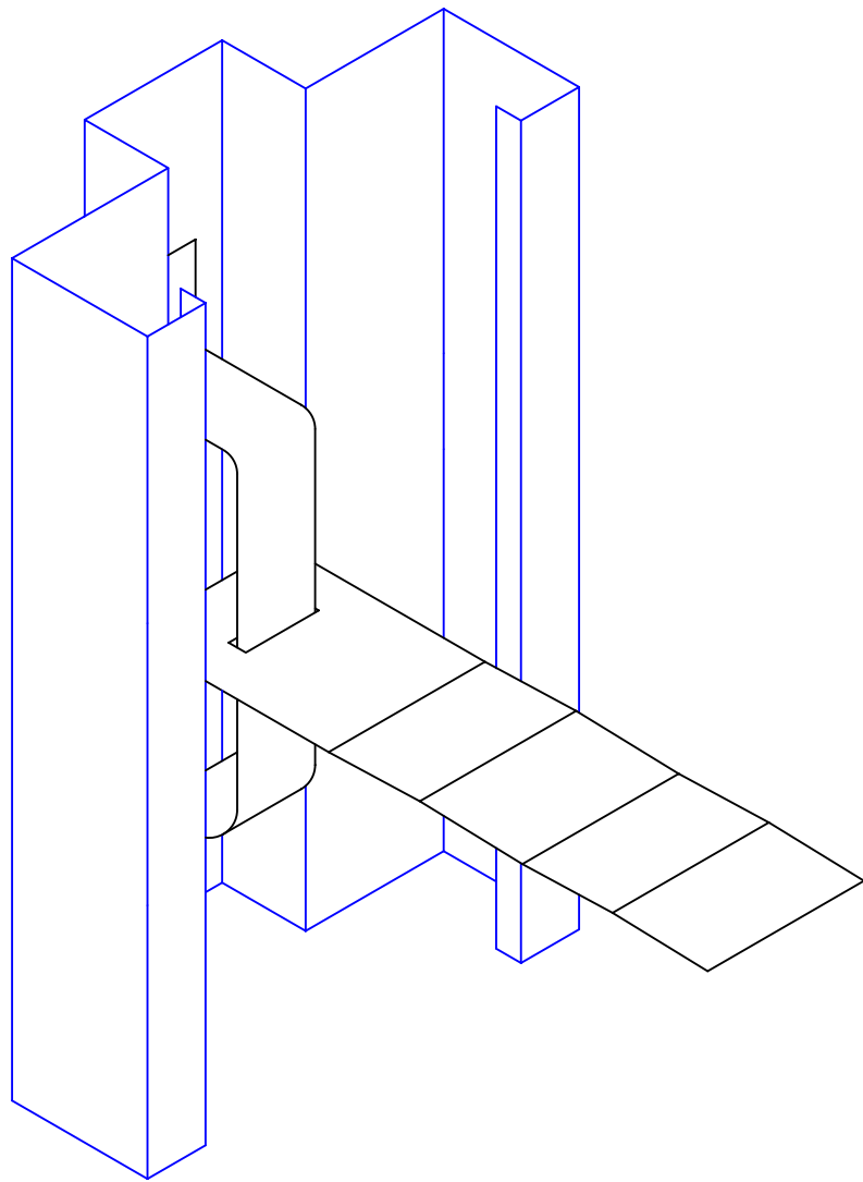
MASONRY JAMB ANCHOR ADJUSTABLE STRAPS W/ WELDED YOKE.
