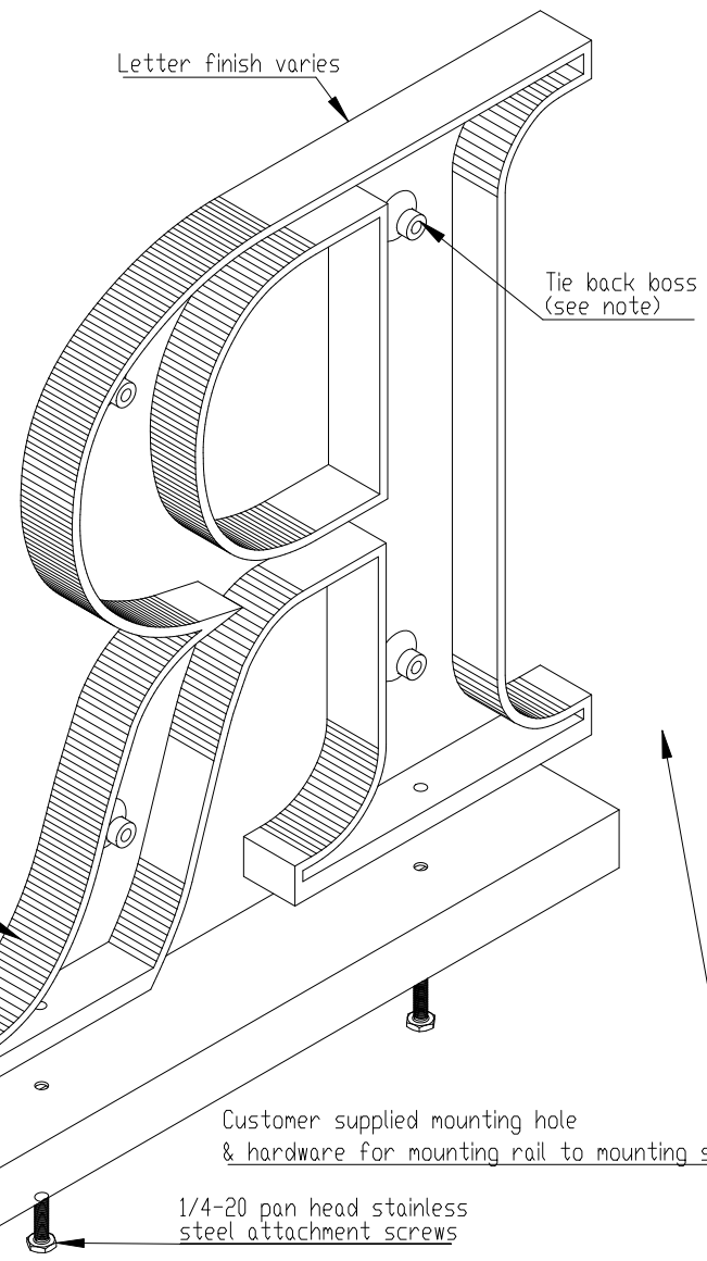
ISOMETRIC BACK VIEW II SCALE 1:3
