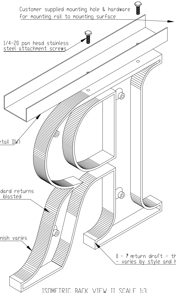
ISOMETRIC BACK VIEW II SCALE 1:3
