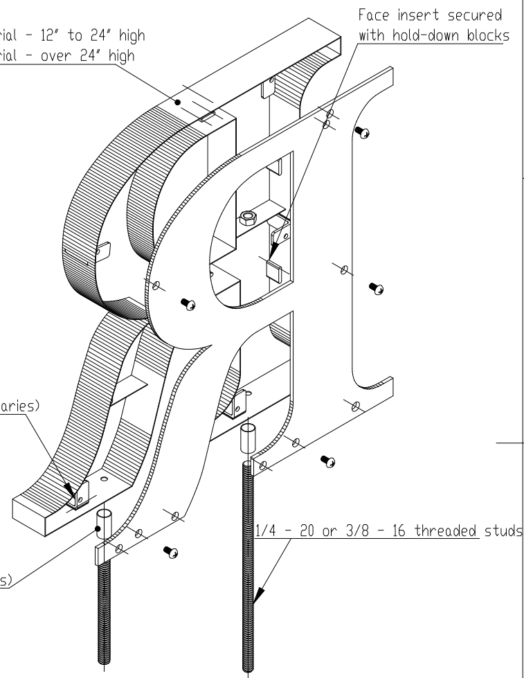
ISOMETRIC BACK VIEW II SCALE 1:4
