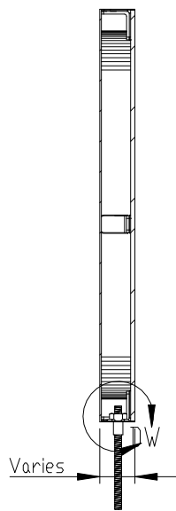
SECTION VIEW A-A II SCALE 1:5
